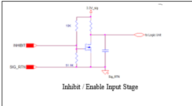
Figure 1 – Inhibit and Enable Input stage
