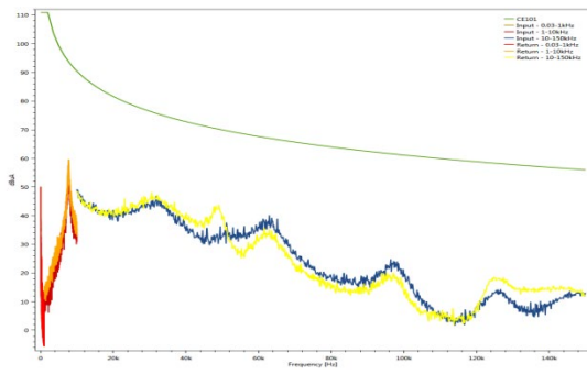
CE101 (30 Hz to 150 kHz)
