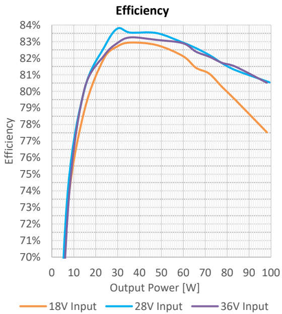
M7009-101 (12 V DC output)
