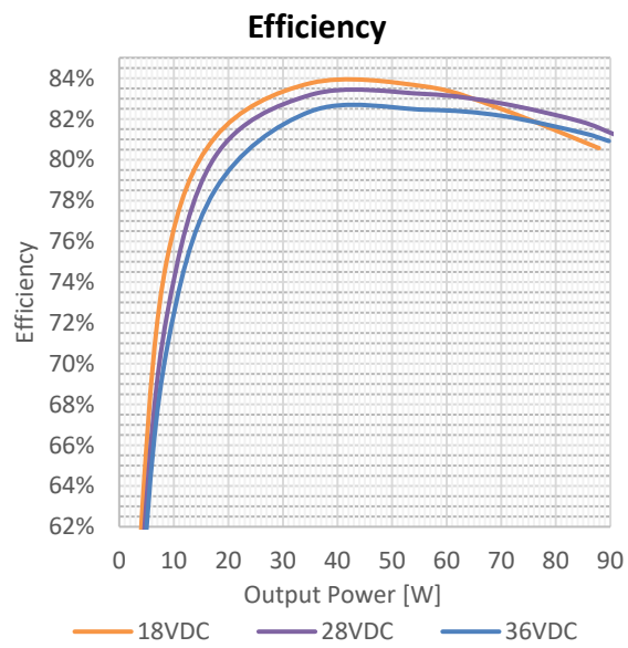
M7009-104 (28 V DC output)
